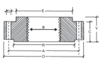
THREADED FLANGES
